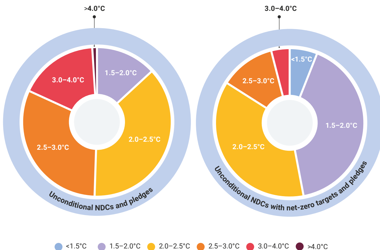
Figure 4.3. Range of global warming outcomes projected if unconditional nationally determined contributions and announced pledges continue (left) and if additionally net-zero targets announced by countries are achieved (right)
