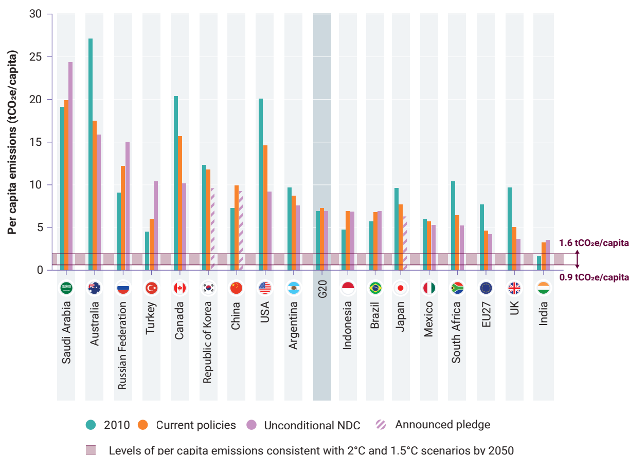
Figure 2.6. Per capita greenhouse gas emissions of the G20 and its individual members by 2030 under nationally determined contributions and other announced 2030 pledges as at 30 September 2021, current policies scenario projections from independent studies mainly published after the COVID-19 outbreak, and 2010 historical levels
